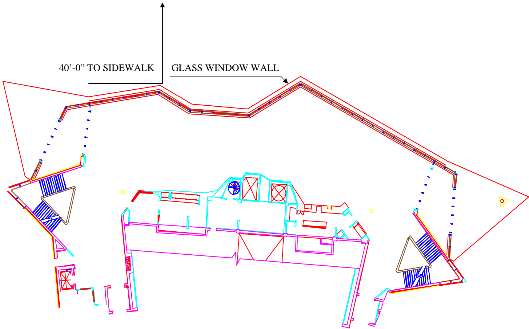
1 GROUND PLAN OF ROZSA LOBBY SCALE: NONE
